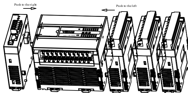
Figure 5-1 Extension module cascading method
