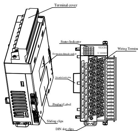
Figure 1-1 I/O expansion module form factor and components
